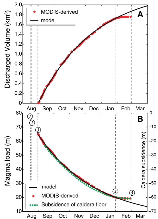
Figure 3. Magma volumes measured during Bárðarbunga-Holuhraun eruption (Iceland) by moderate resolution imaging spectroradiometer (MODIS) (red points) shows fit of R^2 = 0.99 with modeled volume (Equation 7; black line). B: Assuming cylindrical shape for magma reservoir ( r = 3500 \text{ m} ), excess of volume V_e has been then converted to relative change of level of magma in chamber (black line). Shift of -15 \text{ m} is added in order to take into account subsidence that occurred before beginning of effusive eruption. Changes in magma level derived from satellite data (red points) fits perfectly GPS data (corrected for ice flow) tracking subsidence of Bárðarbunga caldera (green dashed line; from Gudmundsson et al., 2016) and gravity-driven model (black line) as predicted by Equation 8. Numbered circles indicate main steps of eruption as labeled in Figure 2.
